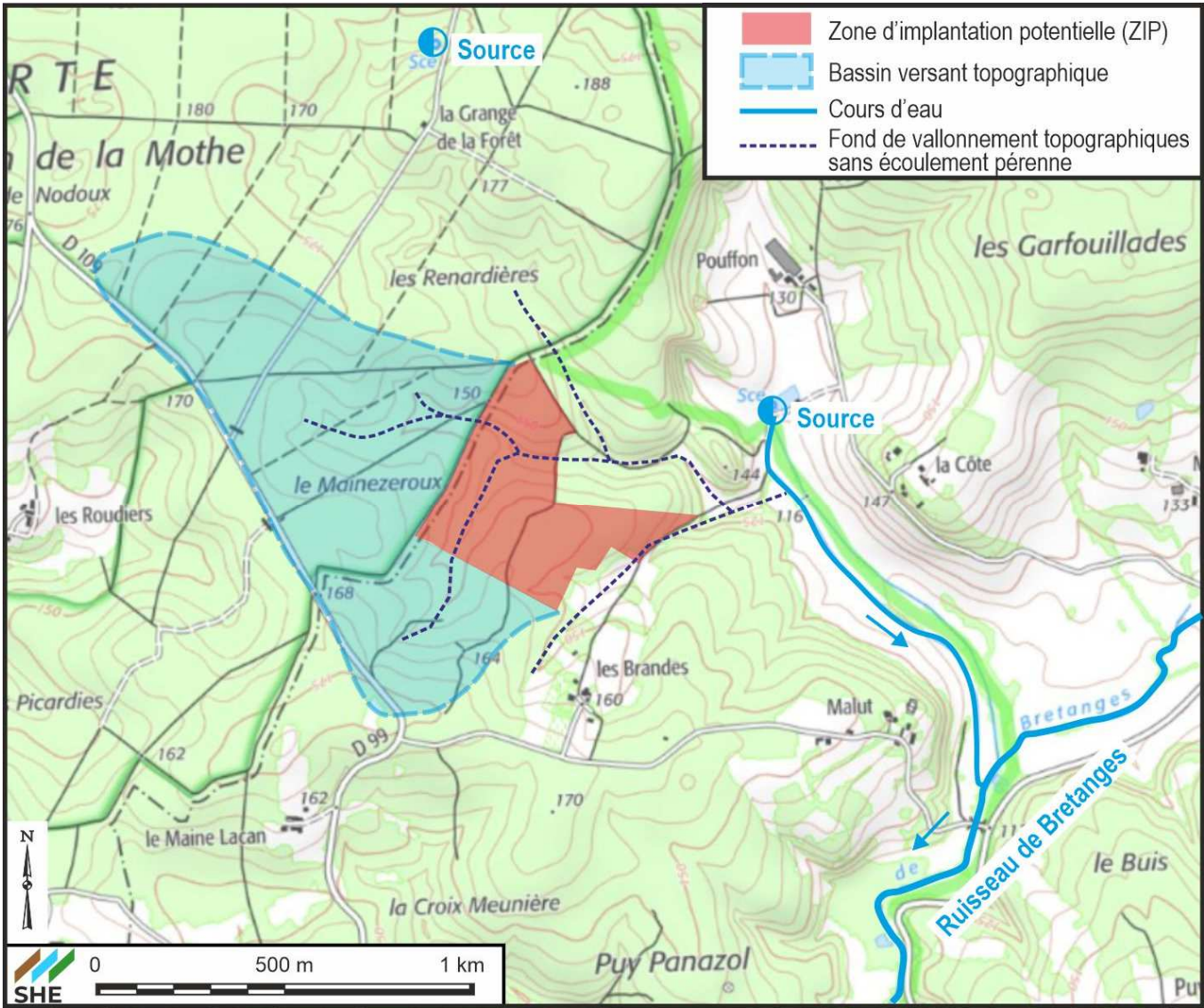
Figure 29 : Hydrologie locale
